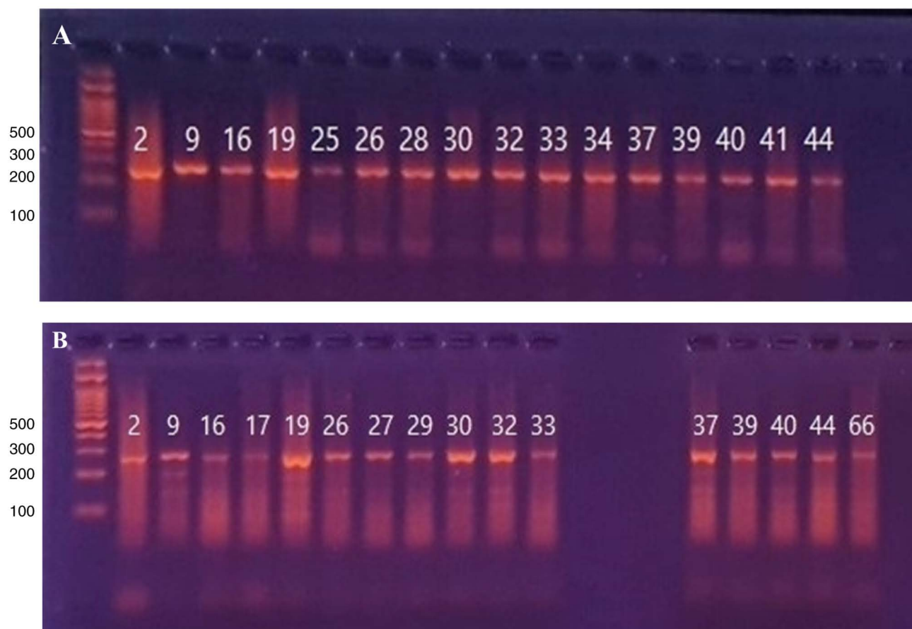
Figure S1. Agarose gel electrophoresis of PCR product for tumor suppressor gene Von Hippel Lindau and kinase insert domain receptor genes. (A) Represent amplification of exon I of VHL gene. (B) Represent the amplification segment of axon 13 of KRD gene. Lane 1: Ladder. Lane 2-16 demonstrate PCR products of ccRCC patients. The bands for both VHL and KRD fragments for all patients were located within the expected fragment size (VHL=260 bp and KDR=290 bp).
